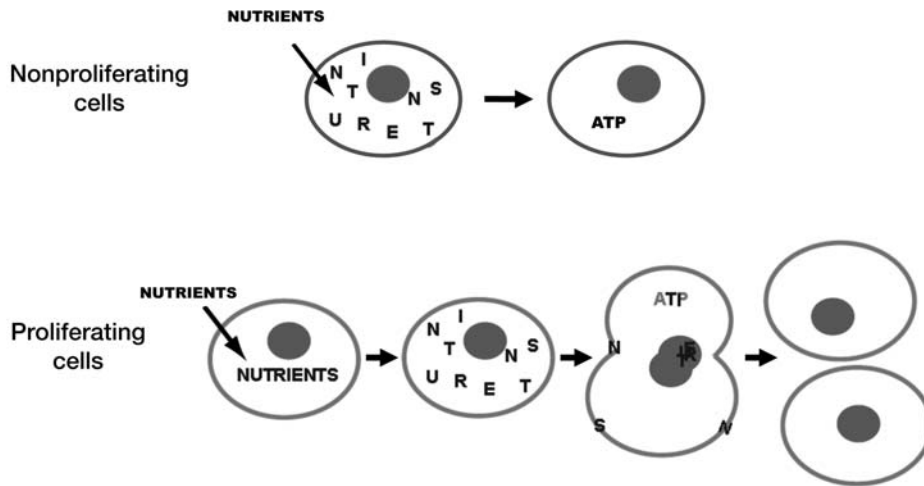
Figure 1. Cell proliferation requires additional nutrient uptake to support duplication of biomass. The otherwise unfavorable reactions required by all cells to maintain homeostasis are coupled to ATP hydrolysis. This requires the constant regeneration of ATP, and as a result all cells rely on nutrients to fuel ATP production. In addition to supporting ATP production, proliferating cells must take up additional nutrients and use those nutrients to generate precursors needed to duplicate the mass of the cell.
