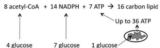
Figure 2. Anabolic metabolism has requirements in addition to ATP. Lipid synthesis to support new membrane production is needed to support the growth and proliferation of many cells. The requirements in terms of carbon units (acetyl-coenzyme A, coA), reducing equivalents (NADPH), and ATP are shown to make a 16-carbon palmitate molecule. Palmitate represents a major structural component of cell membranes. The nutrient "cost" for making each precursor metabolite is shown as a number of glucose equivalents. Even if glycolysis alone is used to generate ATP, fewer than four glucose molecules are needed to make enough ATP for production of a palmitate molecule. The NADPH calculation assumes that two NADPH molecules are generated per glucose via the pentose phosphate pathway. The same glucose molecule can be used to make NADPH and ATP while also generating acetyl-coA, and other pathways and metabolites, such as glutamine, can be used to support lipid synthesis. Nevertheless, the example illustrates that the biosynthesis of many cellular building blocks requires nutrients in excess of those needed for ATP production alone.
